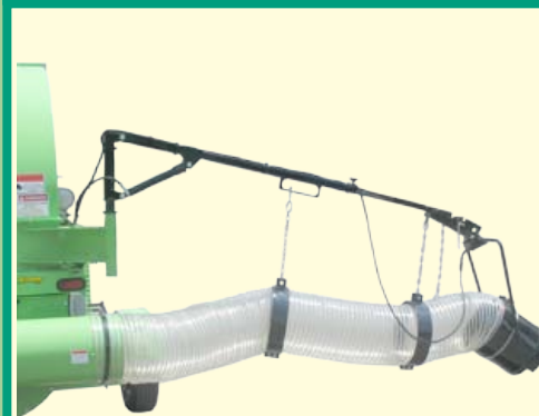
Maneuvering the hose boom is almost effortless because the boom is raised and lowered hydraulically using waterproof switches.
